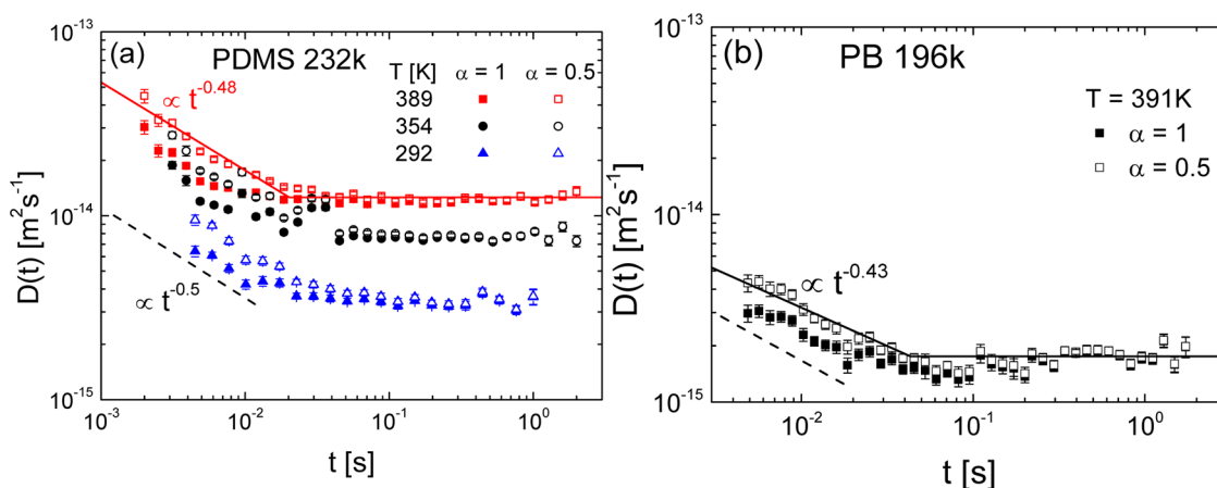
Figure 3. Time-dependent diffusion coefficients of PDMS 232k (a) and of PB 196k (b) as deduced from fits of eq 1 to the measured decay curves S(\tau) as exemplified in Figure 1. For small diffusion times the resulting D(t) depends on the choice of \alpha . The solid lines show fits for highest temperatures and \alpha = 0.5 used in eq 1 (see text) with a power-law decay (resulting exponents are indicated) at short and a constant regime D at long times. The dashed lines illustrate a power law D(t) \propto t^{-0.5} (regime III) predicted by the TR model.
