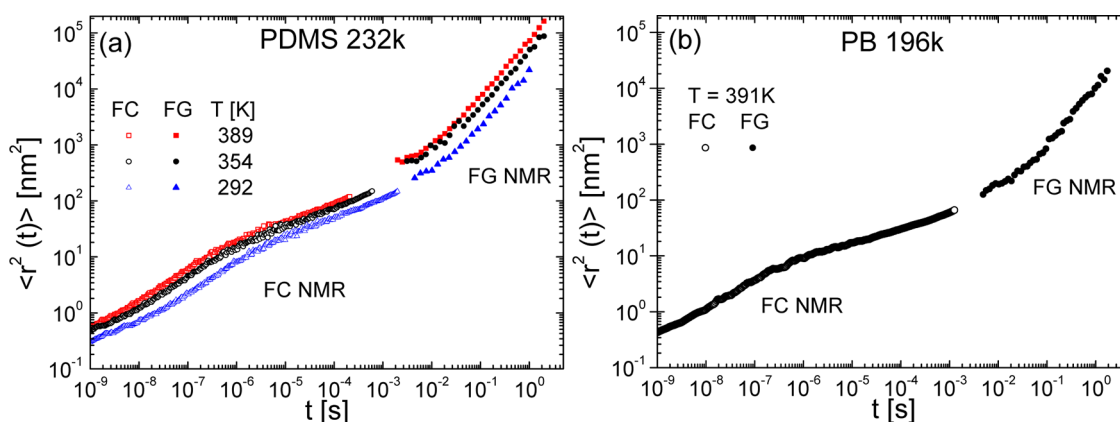
Figure 4. (a) Segmental mean-square displacements obtained from field-cycling (FC) and field-gradient (FG) ^1\text{H} NMR for PDMS 232k at temperatures as indicated. (b) Corresponding results for PB 196k.
